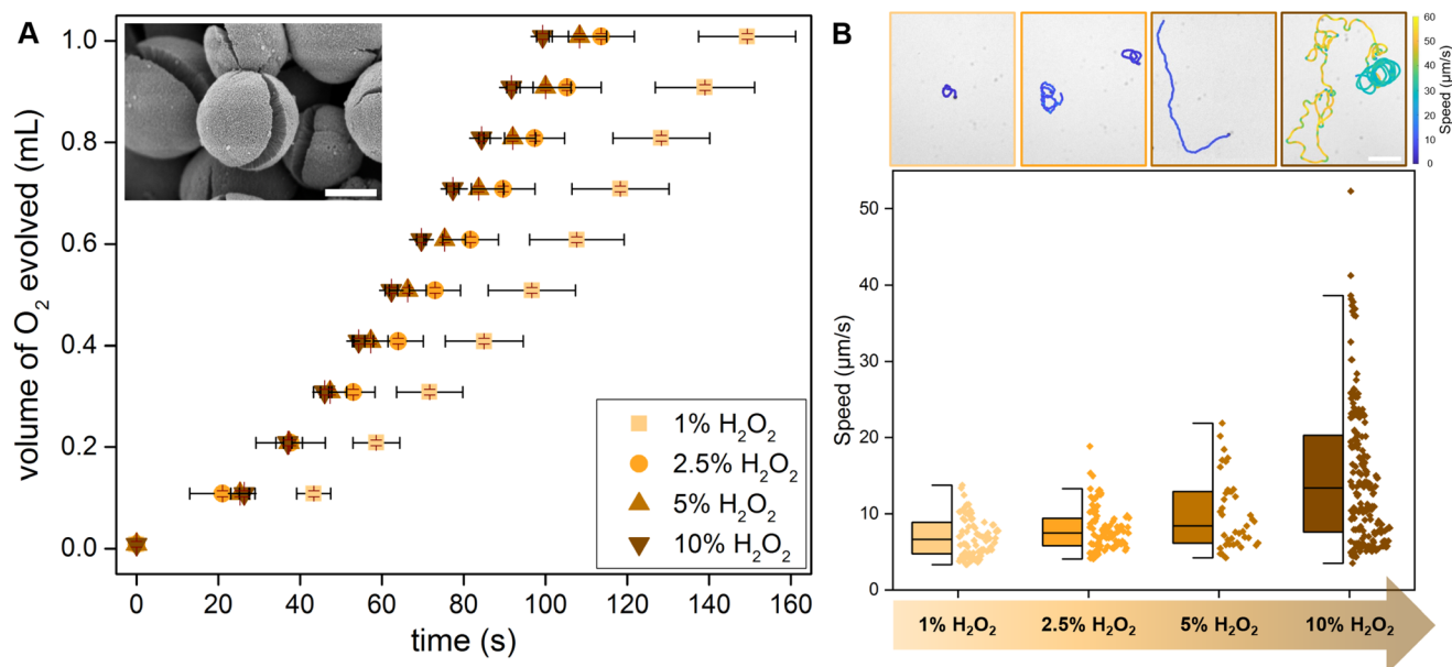
Fig. 2 Correlation between (A) photocatalytic activity of Pac-Man particles measured in terms of time taken to evolve distinct volumes of oxygen and (B) optical images showing trajectories of motion for single particle for 575 frames at different H_2O_2 concentration. The trajectories are color coded according to instantaneous speed and box plots of speed values for at least 40 motile particles for each H_2O_2 concentration. Scale bar in the trajectories is 20 \mu m . Inset in figure (A) shows a SEM image of Pac-Man TiO_2 microparticles, scale bar is 1 \mu m . UV light is used of wavelength 385 nm and intensity 0.25 W cm^{-2} of each LED (total 8 LEDs) and 19.08 W cm^{-2} for oxygen evolution study and microscope experiments respectively.
