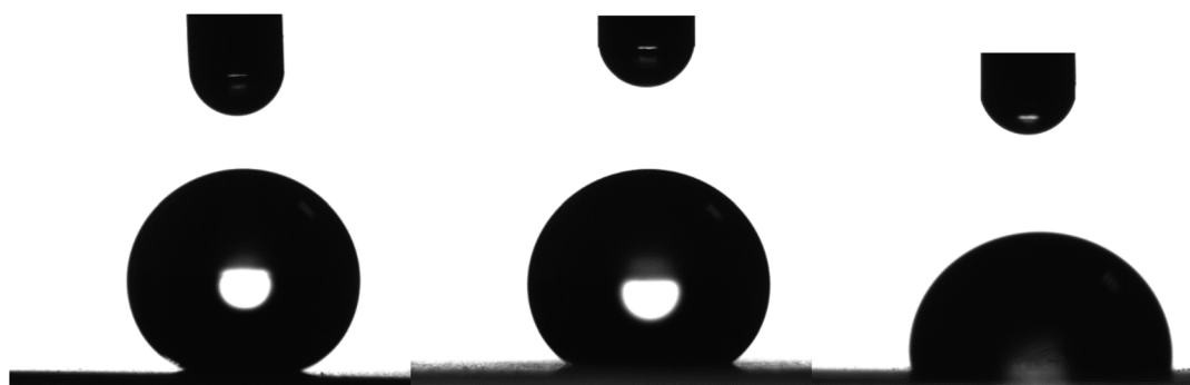
Fig. 16 Photographs of 4 \mu L droplets of (left) glycerol, (center) 1,2-ethylene glycol and (right) DMSO on a LDPE substrate coated with a nano-composite coating containing 56 wt% Dynasylan SIVO 121 and 44 wt% PG003.
