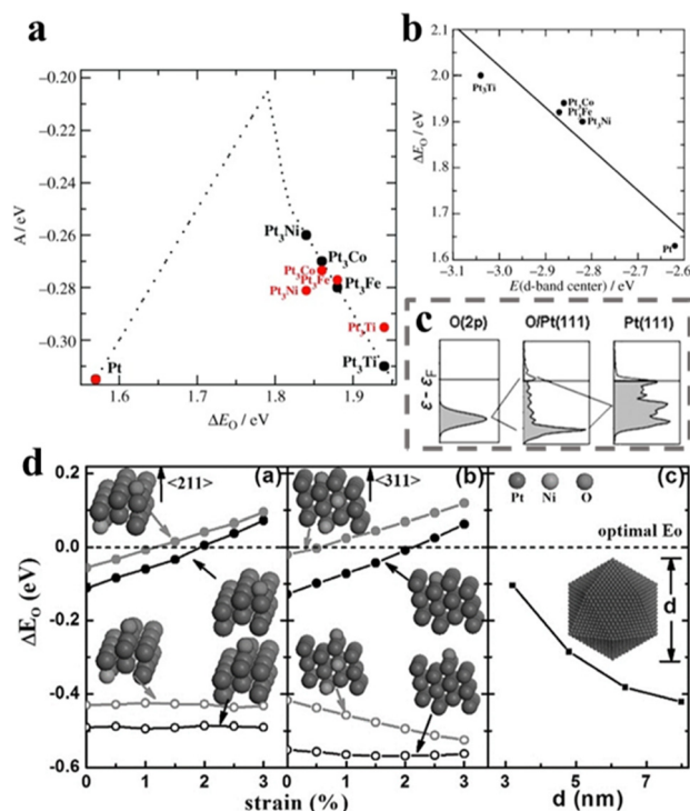
Fig. 25 (a) Model of the activity ( A ) at a cell potential of 0.9 V as a function of the adsorption energy of oxygen, \Delta E_O . The predictions of the model for Pt 3 M ( M = \text{Ni, Co, Fe, Ti} ) alloys are shown relative to the predictions for Pt at the DFT-calculated values of \Delta E_O . (b) The correlation between the d-band center and \Delta E_O . (c) sp-broadened 2p orbital for O(g), projected p density of states of oxygen atoms on Pt(111), and projected d density of states of Pt(111). (d) DFT calculations of oxygen adsorption energy, \Delta E_O as a function of compressive strain on (d(a)) (211) and (d(b)) (311) surfaces. The filled circles represent \Delta E_O values on the hollow sites while the open circles represent the bridge sites. The black and grey curves correspond to \Delta E_O values on pure Pt and Pt 3 Ni surface with top-layer Ni atoms completely removed. (d(c)) \Delta E_O on the (111) facet of the Pt nanoparticles as a function of the particle size. Reprinted with permission from ref. 36 and 39. Copyright 2006 and 2015 from Wiley-VCH GmbH.
