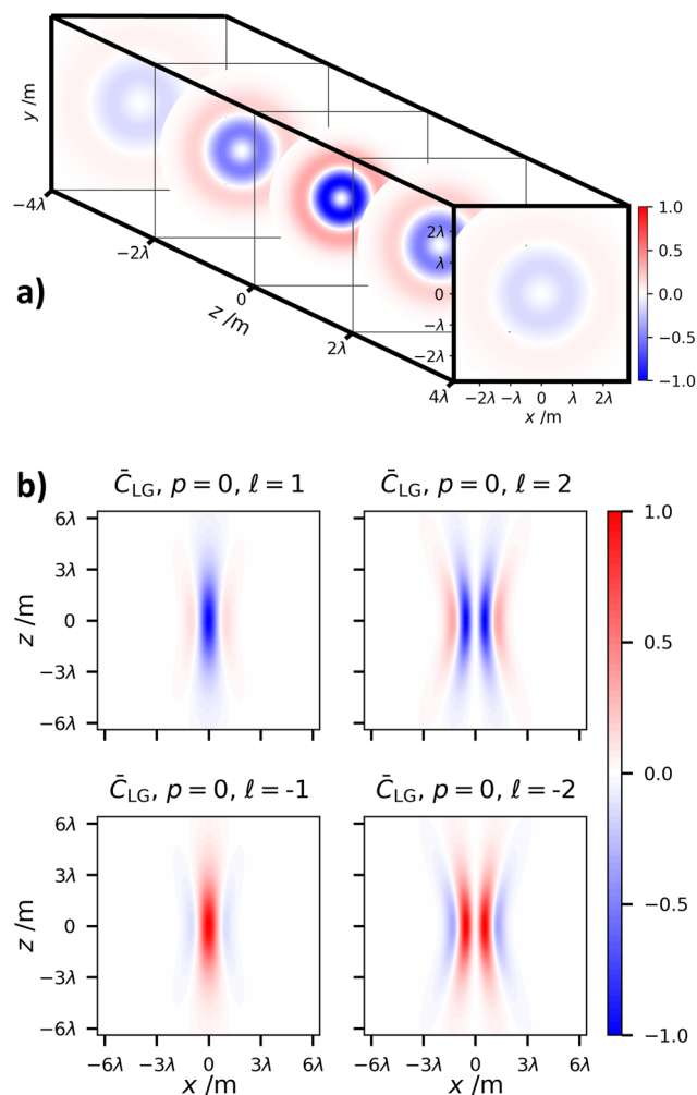
Fig. 9 (a) 3D plot showing the variation of the polarisation independent C_{LG} for a beam with \ell = 2 , p = 0 along the propagation axis. (b) 2D plot showing the diffractive properties of the polarisation independent optical chirality density of LG beams, which stemming purely from longitudinal fields means \bar{C}_{LG} = \bar{C}_{LG}^{\parallel} . In all plots w_0 = \lambda .
