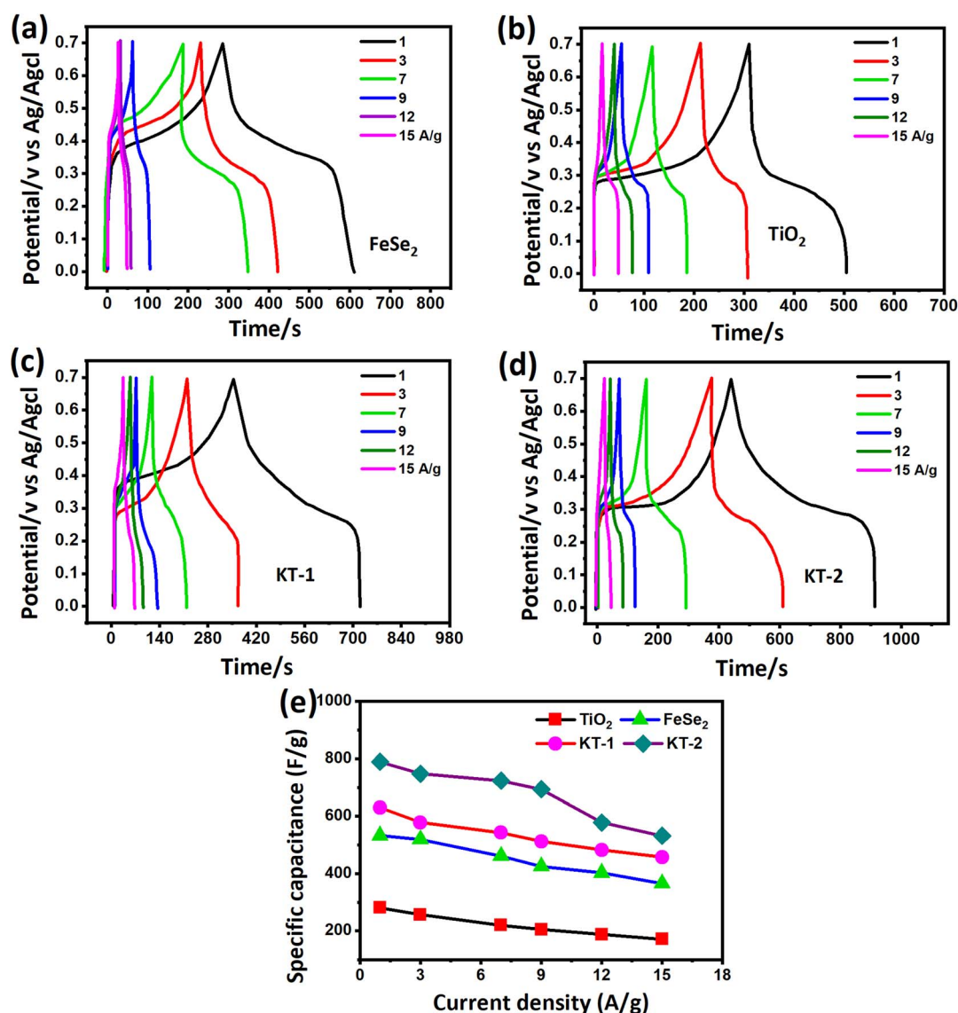
Fig. 6 GCD curves of (a) \text{FeSe}_2 , (b) \text{TiO}_2 , (c) KT-1, (d) KT-2, and (e) comparative capacitance performance of all electrodes at different discharge currents.
