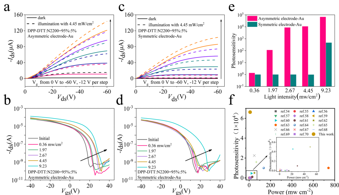
Fig. 3 (a) and (b) Photoresponse performance test of DPP-DTT:N2200 asymmetric electrode devices. (a) Output curves of the device in the dark and under illumination with 4.45 mW\ cm^{-2} light intensity. (b) Transfer curves of the device under different light intensities. (c) and (d) Photoresponse of DPP-DTT:N2200 symmetrical electrode devices. (c) Output curves of the device in the dark and under illumination with 4.45 mW\ cm^{-2} light intensity. (d) Transfer curves of the device under illumination with different light intensities. (e) Photosensitivity of the device under different light intensities. (f) Comparison of the photosensitivity of organic polymer photonic transistors for literature results and this work.
