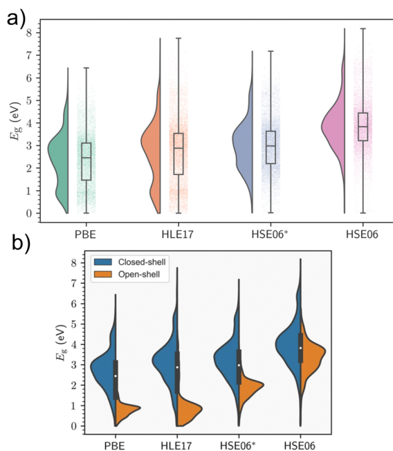
Fig. 13 (a) Distribution of band gaps, E_{\text{g}} , for the 10 720 structures found within the QMOF database, determined using periodic DFT using GGA (PBE), meta-GGA (HLE17), and hybrid (HSE06, HSE06*) functionals, and (b) decomposed into the closed- and open-shell contributions. Adapted with permission figure from ref. 83. IOP Publishing. Reproduced with permission. All rights reserved.
