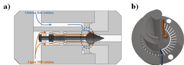
Fig. 2 (a) Schematic representation of the valve-assisted mixer structure. (b) Fluid guidance via the mixing plate. Reprinted with permission from ref. 85. Copyright 2021. American Chemical Society.
