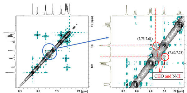
Fig. 5 The NOESY spectrum of 0.2 mg carbazole, 0.2 mg anthracene and 4.0 mg DMF in 400 \mu\text{L} \text{C}_6\text{D}_6 at 8 °C.
