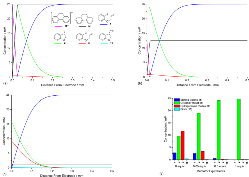
Fig. 6 Influence of mediator (phenanthrene, M ) stoichiometry on reaction layer detachment. Concentration profiles for species 1 , 2 , 3 , 15 , M and M^{\bullet\bullet} for simulated electrolysis under constant potential of -2.8 V vs. SCE at t = 1 s. (a) 1 equiv. of M . (b) 0.5 equiv. of M . (c) 0.05 equiv. of M . (d) Product selectivity profile from simulations with different mediator loadings after electrolysis for 60 s.
