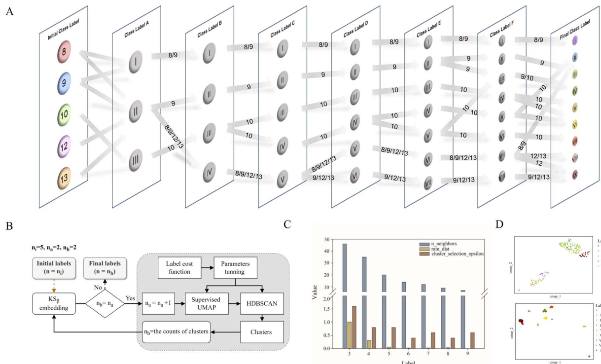
Fig. 2 The flowchart showing the process of \text{KS}_{\beta} labeling (A) and the applications of supervised UMAP and HDBSCAN algorithms (B), the parameter optimizations during the process of A and B (C), and the supervised UMAP comparison of T2PK class labeling generated by five manually annotated class labels (up, D) and nine refined class labels (bottom, D).
