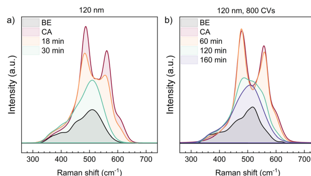
Fig. 2 Overlapped in situ Raman spectra of NiOOH reduction for two 120 nm NiO samples in 1 M KOH: a) before conditioning, in b) the sample was conditioned by 800 CVs to form more Ni(OH) 2 . At 1.50 V vs. RHE (labelled “CA”), vibrations of NiOOH at 480 cm -1 and 560 cm -1 appear. The spectra are overlaid with spectra taken “x min” after stopping chronoamperometry. They show the gradual transformation of the spectral line back to the one characteristic for NiO before electrochemistry (labelled “BE”).
