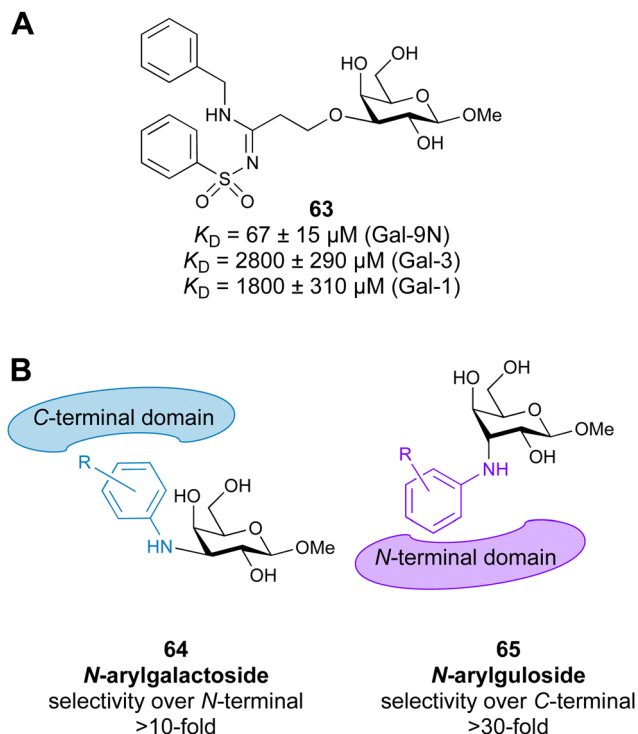
Fig. 12 Gal-9 inhibitors. (A) Galactoside- N -sulfonyl amidine, (B) selectivity switch between 3- N -aryl galactosides and 3- N -aryl gulucosides.
