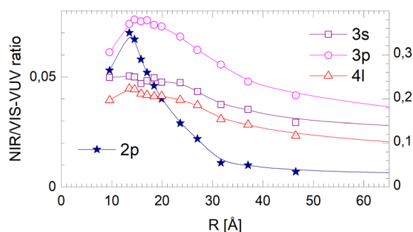
Fig. 17 Dependence of the NIR/VIS – VUV fluorescence intensity ratio on the radius, R , of ^4\text{He} clusters for selected spectral regions (see text). Note the different scales for 2p (left) and 3s, 3p and 4l (right). For 2p-related excitations, the normalised NIR/VIS fluorescence intensity decreases rapidly with cluster size. 3p is an intermediate case. For 3s and 4l the normalised NIR/VIS fluorescence intensity remains almost constant (see text). The range of R is limited to the region that is free from artefacts (see text).
