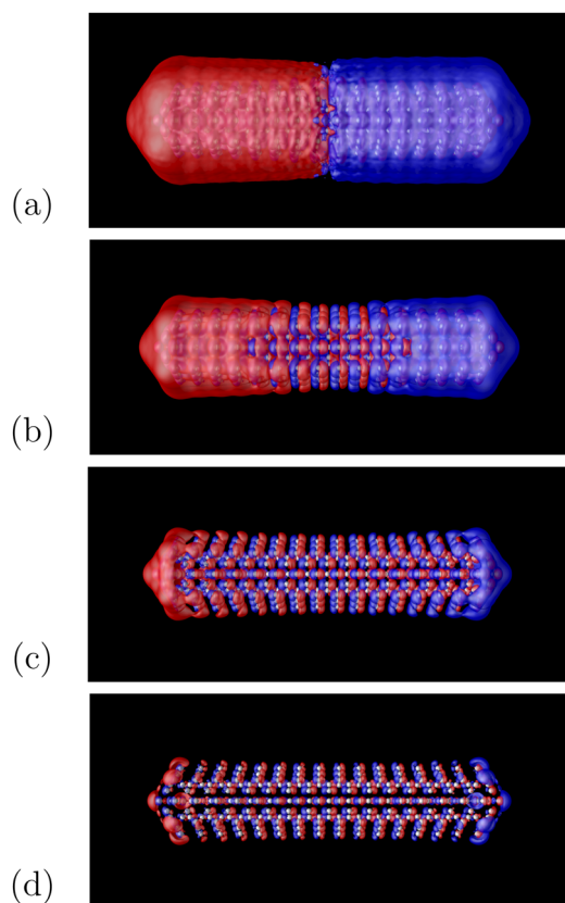
Fig. 4 Induced density of the \text{Ag}_{263} rod after the same optical excitation as shown in Fig. 3, i.e. , showing the oscillation at the plasmon frequency. The density of the isosurfaces is progressively increasing, (a) 1 \times 10^{10} , (b) 1 \times 10^8 , (c) 5 \times 10^8 , and (d) 1 \times 10^7 . The lowest value in (a) highlights the overall dipole mode of the delocalized electrons, whereas with increasing density values, the induced dipoles of the d states around the atoms with opposite polarization become clearly visible.
