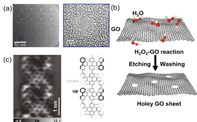
Fig. 4 (a) TEM image of a representative graphene nanopore array and magnified TEM image of a nanopore with an exposure time of 0.1 s. A helium ion beam microscope was used to produce the single-layer graphene. 132 (b) Carbon atoms in the actively defective zones of GO can be oxidized by H 2 O 2 , thereby generating nanopores gradually. 144 (c) AFM image acquired on the graphene nanoribbon segment and a scheme of its chemical structure. 145 Figures adapted with permission from Elsevier, Copyright (2021), Nature Publishing Group, Copyright (2022), and John Wiley and Sons, Copyright (2022).
