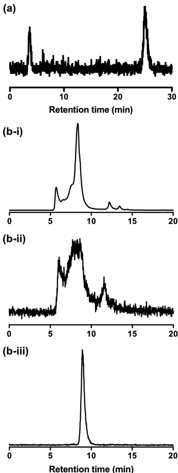
Fig. 5 (a) Reverse phase C 8 HPLC radiochromatogram of [ 111 In]In-DTPA-CTP after incubation in murine serum for 24 h, demonstrating that >70% of [ 111 In]In-DTPA-CTP remained intact with respect to dissociation of [ 111 In]In 3+ from the DTPA chelator. The signal at 4.1 min corresponds to [ 111 In]In 3+ released from DTPA-CTP. (b)–(i) Size exclusion HPLC UV chromatogram of murine serum (280 nm). (b)–(ii) Size exclusion HPLC radio-chromatogram of a solution of [ 111 In]In-DTPA-CTP incubated with murine serum for 24 h. Comparison with the UV chromatogram indicates that [ 111 In]In-DTPA-CTP interacts globally with many serum components. (b)–(iii) Size exclusion HPLC radio-chromatogram of a solution of [ 111 In]In 3+ incubated with murine serum for 24 h, indicating that [ 111 In]In 3+ likely binds specifically to a single serum component.
