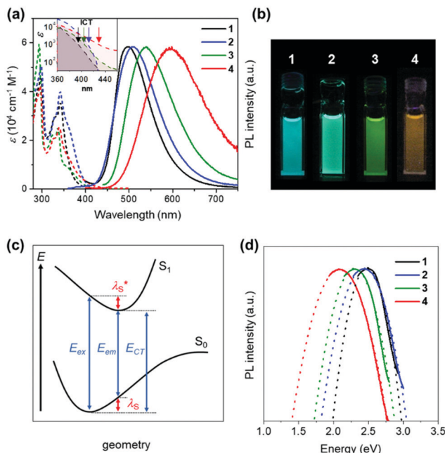
Fig. 3 (a) UV-vis absorption and PL spectra of 1–4 in toluene ( 1 \times 10^{-5} \text{ M} ). The inset shows a magnified view of the ICT absorption bands. (b) Photograph of the PL emissions from the solutions under UV irradiation. (c) Schematic potential energy diagram of the S_0 and S_1 states; E_{\text{ex}} , E_{\text{em}} , and E_{\text{CT}} denote the energies of excitation, emission, and charge transfer, respectively. (d) PL spectra (solid lines) fitted using eqn (1) for the evaluation of \lambda_{\text{S}} .
