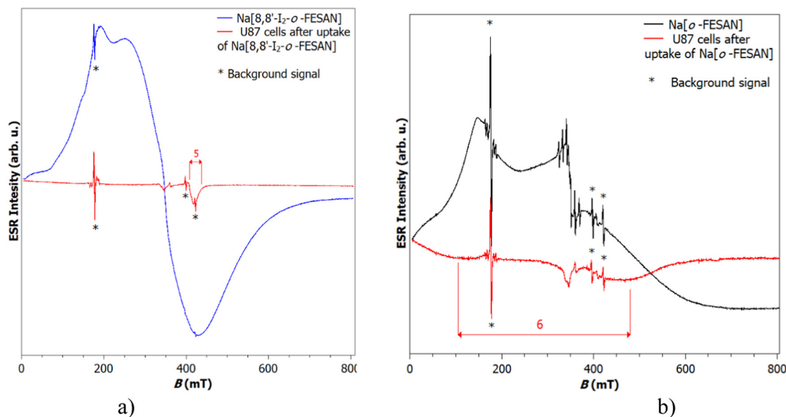
Fig. 1 (a) Spectra of \text{Na}[8,8'\text{-I}_2\text{-o-FESAN}] in powder, U87 cells after uptake of \text{Na}[8,8'\text{-I}_2\text{-o-FESAN}] . The g factor indicated by number 5 is 1.7. (b) Spectra of \text{Na}[\text{o-FESAN}] in powder and U87 cells after uptake of \text{Na}[\text{o-FESAN}] . The g factor indicated by number 6 is approximately 2.
