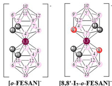
Scheme 1 Schematic representation of the small anionic ferrabis(dicarbollide) clusters with their vertices numbered. Circles in grey correspond to C_{cluster} -H vertices while the pink and the red ones to B-H and B-I vertices, respectively.
