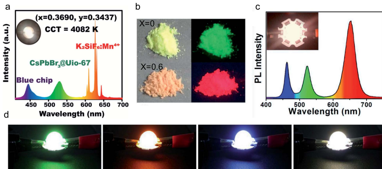
Fig. 8 (a) PL spectra of the as-fabricated WLEDs with the \text{CsPbBr}_3@\text{Uio-67} composite and commercial \text{K}_2\text{SiF}_6:\text{Mn}^{4+} red phosphor deposited on the blue chip (InGaP, 455 nm). Inset: Photograph of the WLEDs. (b) Photographs of \text{CsPbI}_{3-x}\text{Br}_x/\text{MOF-5} powders ( x = 0 and 0.6 ) taken under daylight (left) and 365 nm UV illumination (right). Reprinted with permission from ref. 113. Copyright 2019 American Chemical Society. (c) The corresponding EL spectrum with a photo of the white LED in the inset. Reprinted from ref. 112. Copyright 2019, with permission from Elsevier. (d) Photograph of blue, green, red, and white LEDs, respectively, using Bio-MOF-1 developed by Zhang et al. Reprinted from ref. 108. Copyright 2019, with permission from Elsevier.
