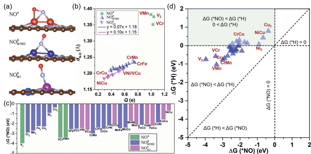
Fig. 2 (a) Side views of the three most stable adsorption configurations of NO over M1M2@NG DACs. (b) The relationship between the charge transfer ( Q , e) and the N–O bond length ( d N–O (*NO), Å) of the most favorable *NO configurations on each M1M2@NG. Here, the positive values of Q indicate electron transfer from the catalyst to the adsorbed NO. (c) The free energy change ( \Delta G (*NO), eV) of the most stable *NO configuration over various DACs. (d) The \Delta G for the *NO and *H over various DACs.
