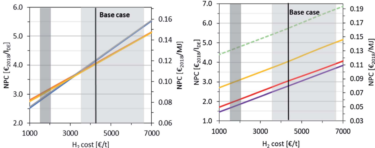
Fig. 11 (Left) Dependence of NPC on the \text{H}_2 cost: — P1, — P2, — P3, — P4 dark grey shaded area: SMR cost range representing a prospective lower limit of green \text{H}_2 cost according to ref. 71 and light-grey shaded area: wind power-based electrolysis cost range from ref. 71. All other raw material costs are fixed on the base case. (Right) Dependence of NPC on the \text{H}_2 and \text{CO}_2 cost: — P4 at 0 \text{€} per t_{\text{CO}_2} (available \text{CO}_2 in-site), — P4 at 62 \text{€} per t_{\text{CO}_2} ( \text{MEA}_{2018} cost from ref. 68), — P4 base case, - - P4 at 720 \text{€} per t_{\text{CO}_2} ( \text{DAC}_{2018} cost from ref. 70); dark grey shaded area: SMR cost range representing a prospective lower limit of green \text{H}_2 cost according to ref. 71, light-grey shaded area: wind power-based electrolysis cost range from ref. 71.
