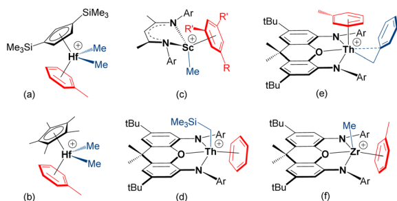
Fig. 1 Crystallographically-characterized early transition metal and f-element alkyl cations which exist as arene-solvent-separated ion pairs ( \text{R} = \text{Me} or \text{Br} and \text{R}' = \text{H} , or \text{R} = \text{R}' = \text{Me} ; \text{Ar} = \text{C}_6\text{H}_3\text{Pr}_2\text{-2,6} or \text{C}_6\text{H}_2\text{Pr}_3\text{-2,4,6} ). 8,10,13,14,18–20
