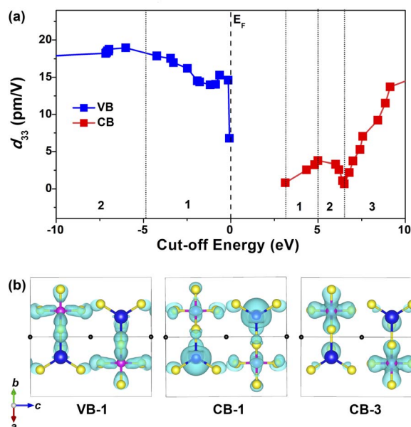
Fig. 7 Theoretical analysis of the SHG source for SrCdSi 4 : (a) variation of cut-off energy (eV) versus the largest static d_{33} ; (b) charge-density-plots in the selections (VB-1, CB-1, CB-3) of major contribution. Black atoms: Sr; blue atoms: Cd; pink atoms: Si; yellow atoms: S.
