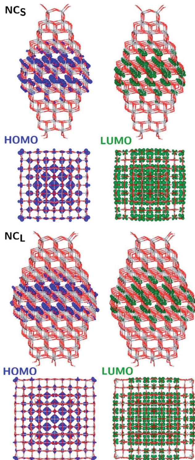
Fig. 10 Side (upper) and top (lower) views of the electronic density plots of the frontier orbitals of NC s and NCL (isosurface = 5 \times 10^{-4} au). Reprinted with permission from G. Fazio, L. Ferrighi and C. Di Valentin, J. Phys. Chem. C , 2015, 119 , 20735–20746. Copyright 2015 American Chemical Society.
