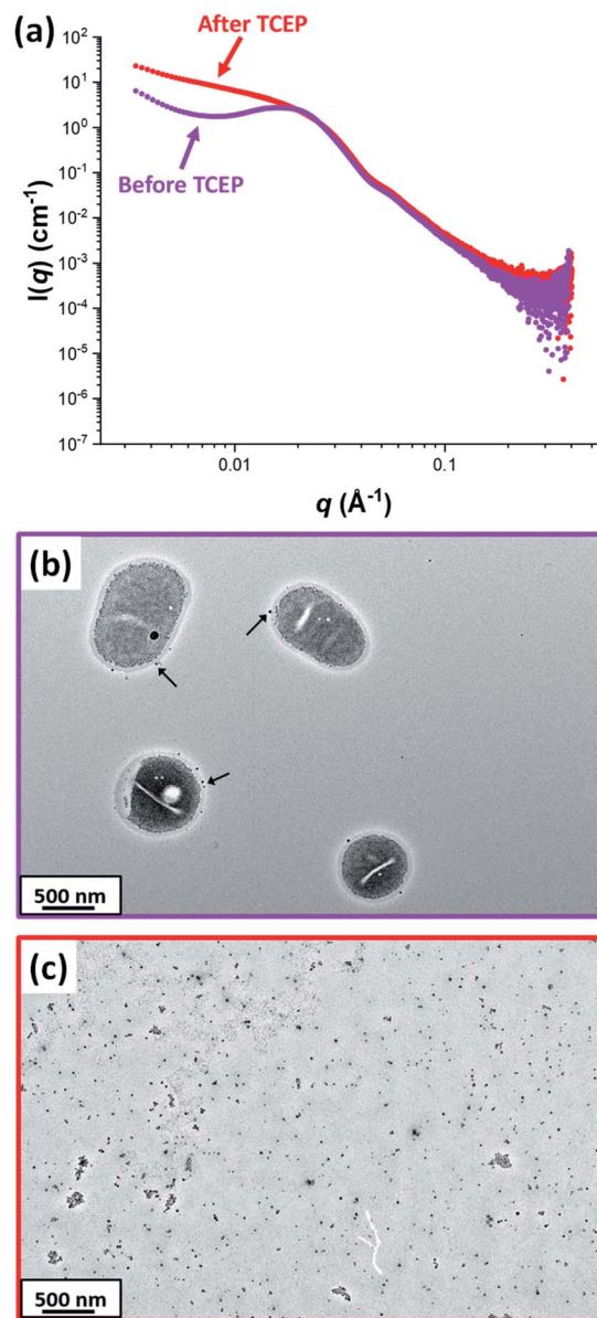
Fig. 7 (a) SAXS patterns recorded for a 1.0% w/w aqueous dispersion of PDMAC_{49} -P(HBA- stat -DAAM) _{302} vesicles (loaded with 2.5% w/w silica nanoparticles) before (purple pattern) and after TCEP addition (red pattern) confirming loss of the structure factor corresponding to the silica nanoparticles encapsulated within the vesicles. The low q gradient in the SAXS pattern recorded at 20 °C indicates the formation of worms after decrosslinking. Corresponding TEM images recorded (b) before and (c) after TCEP addition confirm the presence of silica-loaded vesicles and free silica nanoparticles, respectively. The black arrows shown in (b) indicate a few silica nanoparticles apparently adsorbed to the outer surface of the vesicles. [N.B. The linear worms formed at 20 °C in (c) cannot be observed by TEM because they undergo film formation during TEM grid preparation].
