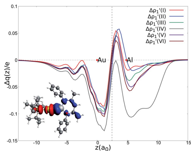
Fig. 2 Charge Displacement (CD-NOCV) curves associated with the \Delta\rho'_1 NOCV deformation density for the interaction between doublet [Bu_3PAu]^\cdot and [X]^\cdot ( X = I-VI ) fragments for complexes [Bu_3PAuX] . Red dots indicate the average position of the nuclei along the z axis. The black dashed line indicates the average position of the isodensity boundary. Positive (negative) values of the curve indicate right-to-left (left-to-right) charge transfer. Inset : isodensity surfaces associated with the \Delta\rho'_1 NOCV deformation density for complex [Bu_3PAuIV] . Charge flux is red-to-blue. Isodensity value is 1 \text{ me a}_0^{-3} . Results for [Bu_3PAuI] and [Bu_3PAuII] are taken and adapted from ref. 33 and 45, respectively.
