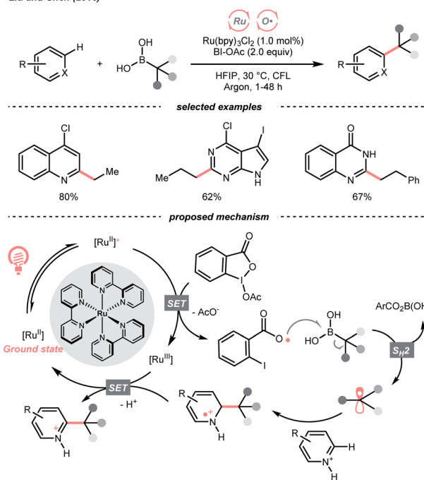
Scheme 49 R • formation via S H 2 of alkyl boronic acid.
