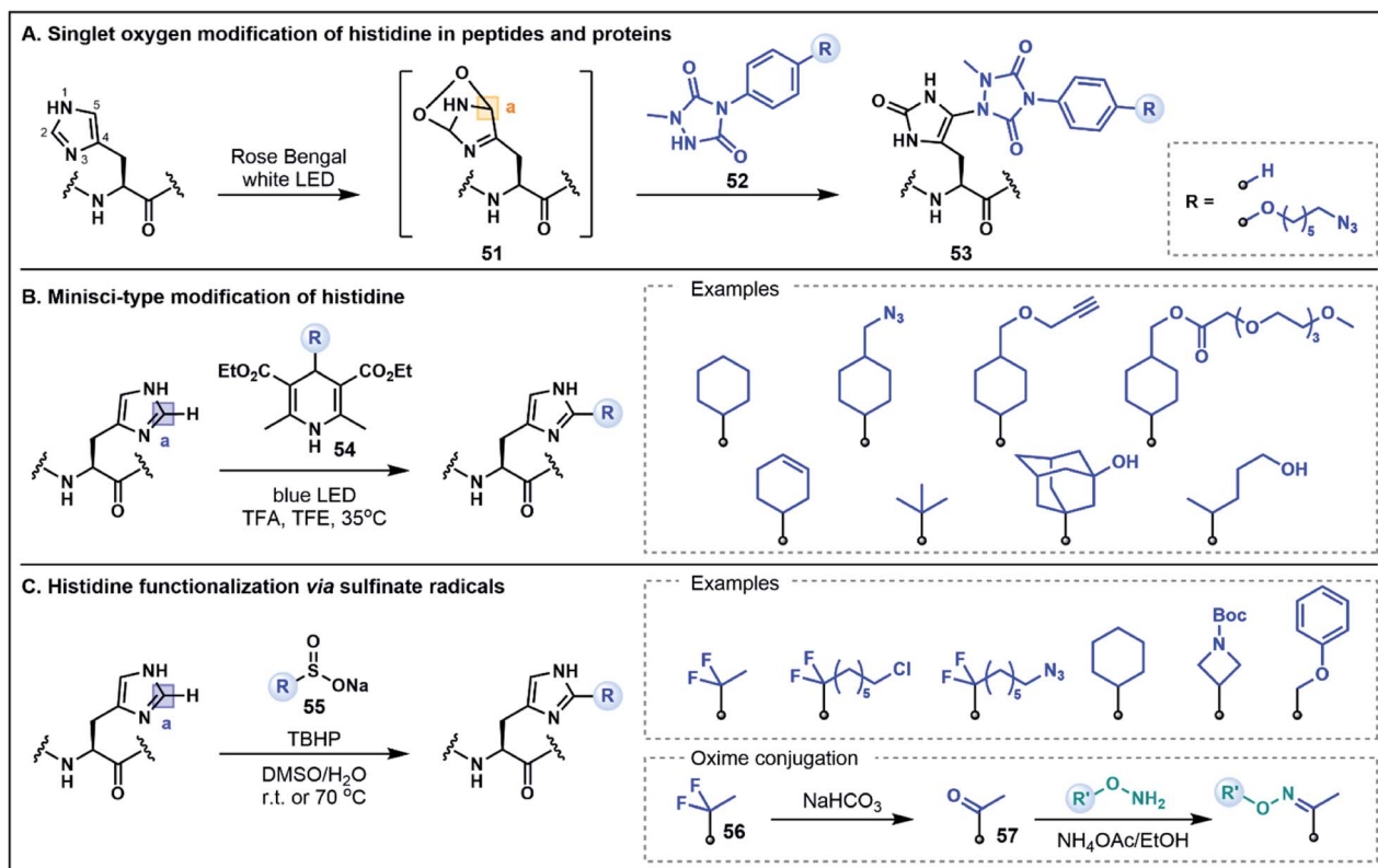
Fig. 8 His functionalization using umpolung-like strategies. (A) Singlet oxygen photooxidative functionalization using 1-methyl-4-aryltriazole nucleophiles. (B) Minisci-type functionalization of His using photochemically generated alkyl radicals. (C) His functionalization using sulfinate salts as radical precursors.
