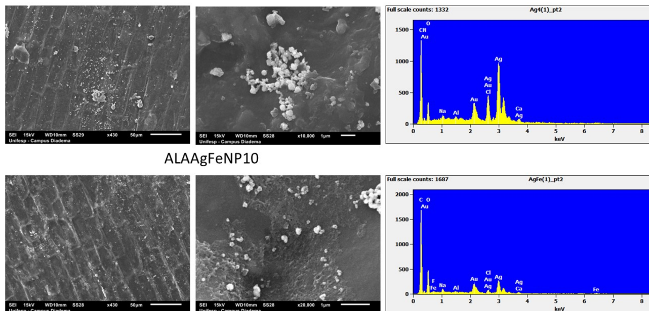
Fig. 4 (a) Optical images of E. densa treated with water, ALA1, ALAAgNP7, ALAAgFeNP10, ALAAgNP6, ALAAgFeNP3 (objective 100×). (b) Scanning electron microscopy images for ALAAgNP7 and ALAAgFeNP10 (50 μm and 1 μm scales) and energy dispersive spectroscopy (EDS) indicates the presence of silver in leaves.
