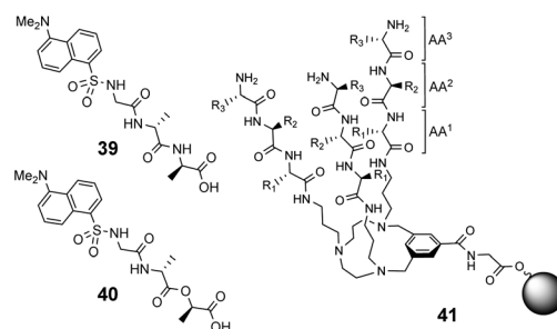
Fig. 15 Dansyl-labelled probes 39 and 40 and vancomycin mimetic combinatorial library 41 containing triazacyclopentane (TAC)-based tripeptides attached to O-glycine functionalised ArgoGel TM resin.
