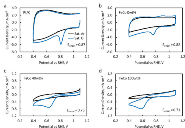
Fig. 10 CVs of (a) a Pt/C reference, (b) FeCo 0 wt%, (c) FeCo 40 wt% and (d) FeCo 100 wt% in a saturated Ar electrolyte (black line) and a saturated O 2 electrolyte (blue line). Scan rate was 50 mV s -1 , in 1.0 M KOH with a stationary RDE.
