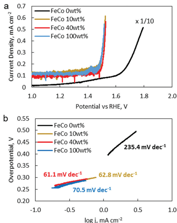
Fig. 9 (a) LSVs of FeCo 0 wt% (black), FeCo 10 wt% (gold), FeCo 40 wt% (red), and FeCo 100 wt% (blue) from 1.0 V to the onset of the OER, in 1.0 M KOH, sat. Ar, at 1600 rpm, at a scan rate of 1 mV s -1 . (b) Tafel slopes derived from polarisation curves in (a). Overpotential is calculated from the thermodynamic potential of the OER (1.23 V vs. SHE).
