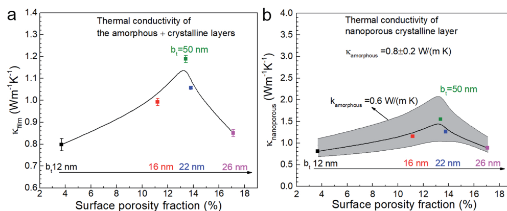
Fig. 9 (a) Effective thermal conductivity \kappa_{\text{film}} of \text{Ca}_3\text{Co}_4\text{O}_9 films as a function of surface porosity fraction, and (b) thermal conductivity of the nanoporous crystalline \text{Ca}_3\text{Co}_4\text{O}_9 layer \kappa_{\text{nanoporous}} , assuming \kappa_{\text{amorphous}} = 0.8 \text{ W m}^{-1} \text{K}^{-1} with a \pm 0.2 \text{ W m}^{-1} \text{K}^{-1} uncertainty captured by error bars.
