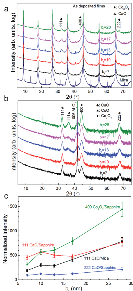
Fig. 1 X-ray diffractograms from as-deposited \text{CaO}/\text{Co}_3\text{O}_4 multilayers with different bilayer thicknesses b_t on (a) mica (001), and (b) sapphire (006) substrates. (c) \text{CaO} and \text{Co}_3\text{O}_4 peak intensities normalized with the intensity of the corresponding substrate peak, plotted as a function of b_t .
