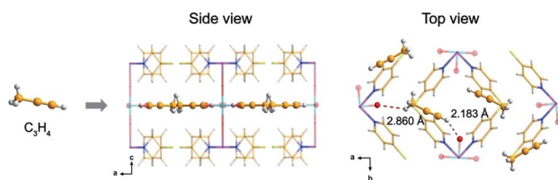
Fig. 9 Schematic diagram of GeFSIX-dps-Cu after adsorbing \text{C}_3\text{H}_4 . 69 Reproduced from ref. 69 with permission, copyright John Wiley and Sons, 2020.
