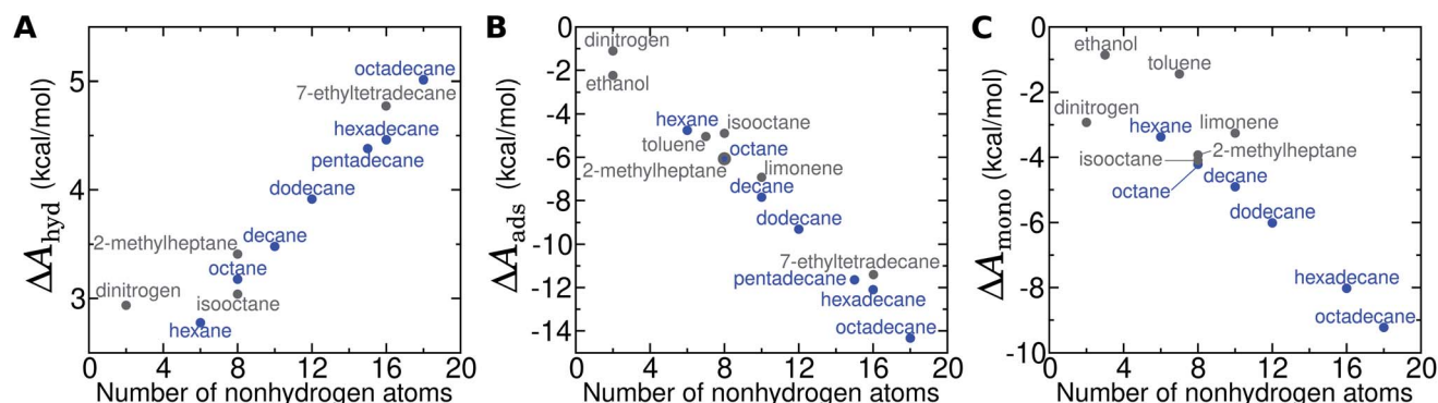
Fig. 8 Adsorption thermodynamics at the graphene–water interface for VOCs and N _2 . (A) Hydration free energy ( \Delta A_{\text{gas} \rightarrow \text{aq}} ) as a function of the number of heavy atoms. Straight-chain alkanes are indicated in blue, while other compounds, including branched alkanes are indicated in gray. For legibility, ethanol, toluene, and limonene have been left outside of the range this graph due to their much more favorable \Delta A_{\text{gas} \rightarrow \text{aq}} values. (B) Free energy of adsorption to the graphene–water interface from aqueous solution ( \Delta A_{\text{aq} \rightarrow \text{ads}} ) as a function of the number of heavy atoms. (C) Free energy of transfer from the adsorbed 2D gas phase to the adsorbed monolayer phase ( \Delta A_{\text{ads} \rightarrow \text{mono}} ) as a function of the number of heavy atoms.
