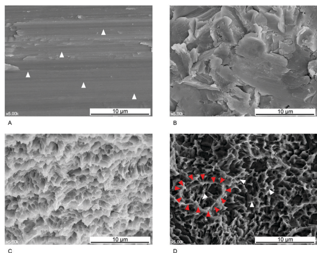
Fig. 3 (A) Scanning electron microscopy (SEM) image of turned Ti. The process of machining via computer numerical control milling yields characteristic grooves (white arrowheads). (B) SEM image of a blasted Ti surface. Many irregularities are formed during the blasting procedure. The surface morphology is affected by the diameter of the blast media (here, approximately 50 \mu\text{m} ), the type of media (here, \text{Al}_2\text{O}_3 ), and the blasting pressure. In general, the irregularities are larger than those formed during etching. (C) SEM image of a Ti surface modified by acid etching showing small honeycomb-shaped irregularities resulting from the etching process. (D) Ti surface sandblasted with large particles (here, approximately 75 \mu\text{m} ), followed by acid etching (Deep Implant System, Inc., Seongnam, Korea) imaged by SEM. The irregularities include large crater-like structures created during the blasting process (red arrowheads) and small honeycomb-shaped micropits (white arrowheads) produced by application of acids to the surface.
