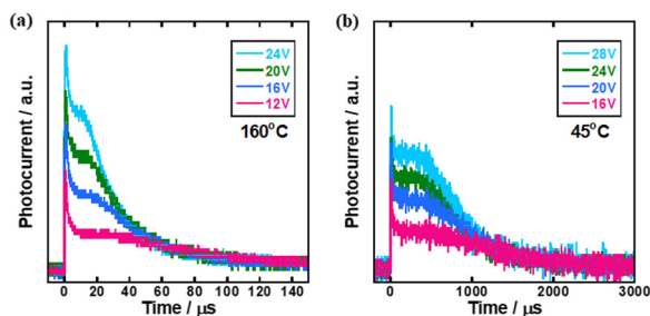
Fig. 6 Transient photocurrent curves for holes (a) in the N* phase of the mixture of compounds 1–3 at 160 °C and (b) in the glassy N* phase at 45 °C. The sample thickness was 4 \mu\text{m} and the wavelength of excitation light was 356 nm.
