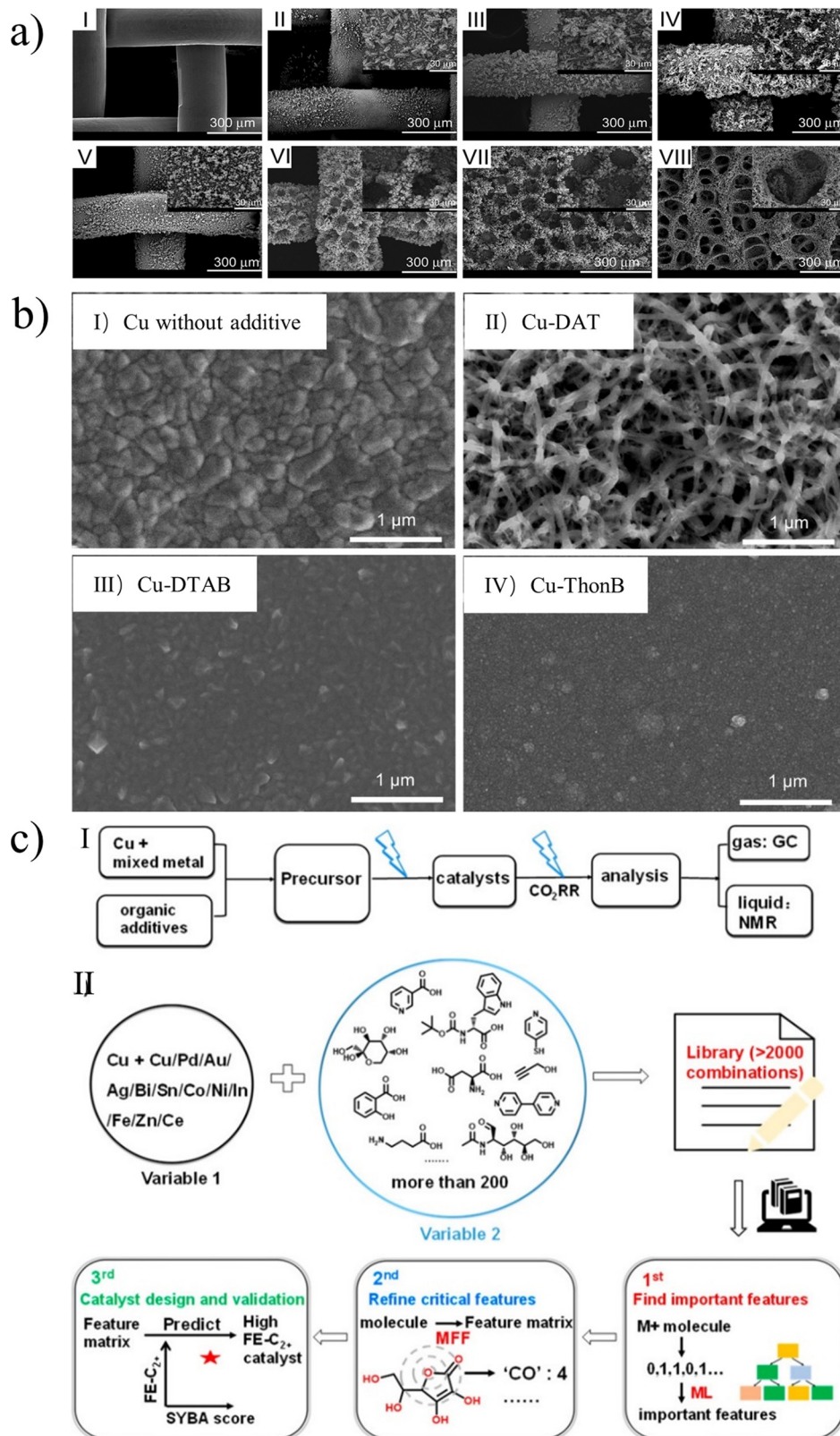
Fig. 6 (a) SEM images of copper electrodes prepared by electrodeposition at different potentials. Reproduced with permission. 36 Copyright 2013, Elsevier. (b) SEM images of Cu electrocatalysts prepared (I) without additive, (II) with DAT, (III) with dodecyltrimethylammonium bromide (DTAB), and (IV) with thonzonium bromide (ThonB). Reproduced with permission. 37 Copyright 2017, American Chemical Society. (c) (I) Preparation of Cu electrocatalysts via electrochemical deposition followed by evaluation of catalytic performance. (II) Schematic illustration of machine-learning-guided optimization of additives for copper catalyst preparation. Reproduced with permission. 43 Copyright 2021, American Chemical Society.
