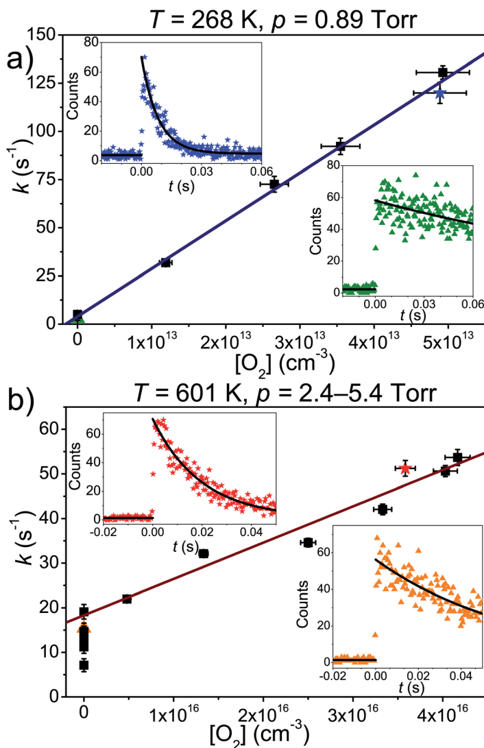
Fig. 2 Examples of bimolecular plots at (a) 268 K and (b) 601 K. The radical traces shown in the upper left and bottom right corners were recorded in the presence and absence of O_2 , respectively. In both figures, the coloured symbols depict the measurements that correspond to the shown traces. Above 500 K, the fitted and measured wall rates do not match. Possible reasons for this are discussed in the Results and discussion section.
