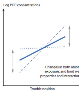
Fig. 1 Conceptual figures showing the concentrations of POPs in relation to trophic position, in the case that climate change influences (top) food web properties or interactions, (middle) abiotic exposures, or (bottom) both food web properties/interactions and abiotic exposures. The solid line represents the present log-normal relationship between the trophic position of the organisms and accumulated contaminant concentrations, while dotted lines reflect the projected window of biomagnification because of the influence of climate change. NAO = North Atlantic Oscillation; TL = trophic level.
