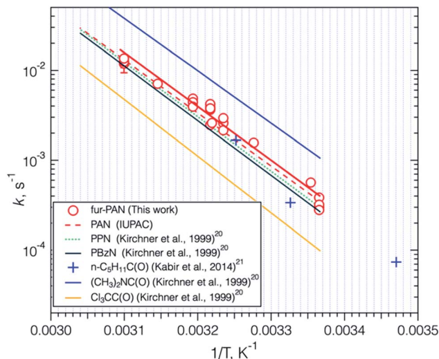
Fig. 6 Arrhenius plot of the thermal decomposition of fur-PAN compared to a number of other acyl peroxyoxynitrate compounds. The individual data points are shown as open circles, with error bars for individual data points, and the fit to the Arrhenius expression is shown as a solid red line. Examples of other Arrhenius expressions are given as noted in the legend, with either the common acronym, or acyl radical, specified.
