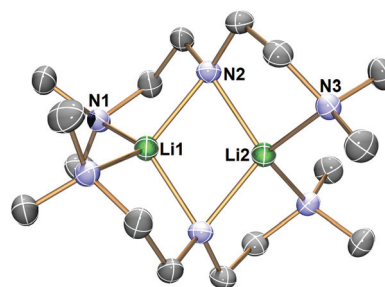
Fig. 3 X-ray crystal structure of [Li(μ- \kappa^2\text{-}N,N'\text{-}N(\text{CH}_2\text{CH}_2\text{NMe}_2)_2 )] 2 ( 2 ) at −123 °C with 50% probability ellipsoids. Hydrogen atoms are omitted for clarity. The selected bond distances (Å) and angles (°) are: Li1–N1 2.0903(18); Li1–N2 2.0286(19); Li2–N2 2.0192(18); Li2–N3 2.0864(17); Li1...Li2 2.376(4); Li1–N2–Li2 71.89(9).
