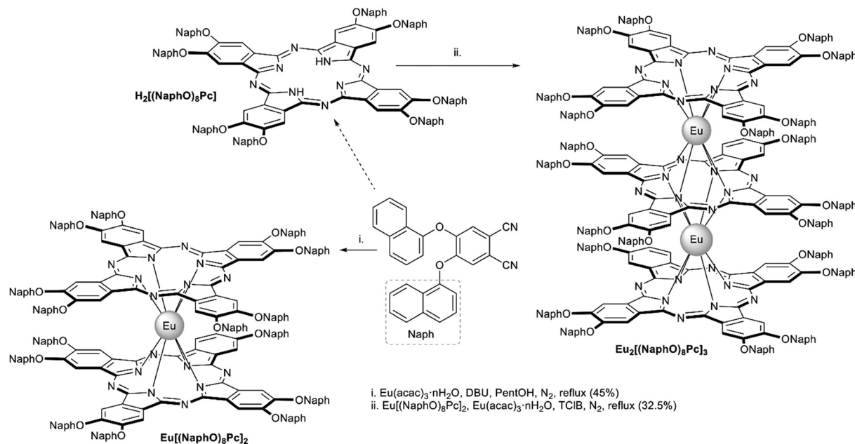
Scheme 1 Synthesis of \alpha -naphthyloxy-substituted \text{Eu}(\text{III}) bis- and trisphthalocyaninates. 38,40
