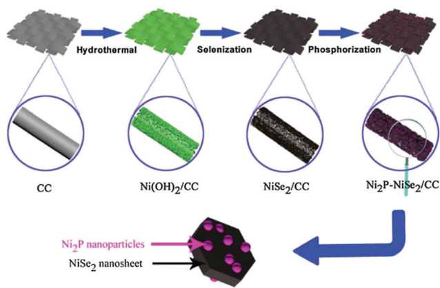
Fig. 81 Schematic illustration of synthesis of \text{Ni}_2\text{P-NiSe}_2/\text{CC} hetero-structure catalyst. Reproduced with permission from ref. 1188 Copyright Elsevier 2020.
