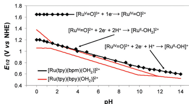
Fig. 120 Plots of E_{1/2} (V vs. NHE) vs. pH for the Ru(v/iv) and Ru(iv/iii) redox couples of [Ru(tpy)(bpm)(OH 2 ) 2+ and for the Ru(v/iii) and Ru(III/II) redox couples of [Ru(tpy)(bpy)(OH 2 ) 2+ in aqueous solution (I) 0.1 M; T) 298 K; glassy carbon working electrode). Reprinted with permission from ref. 1479 Copyright 2008. American Chemical Society.
