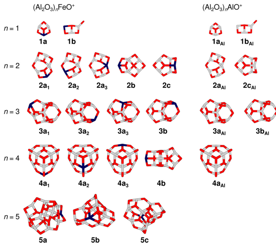
Fig. 2 Overview of TPSSH/def2-TZVP low-energy isomers of (\text{Al}_2\text{O}_3)_n\text{FeO}^+ (left-hand side) and (\text{Al}_2\text{O}_3)_n\text{AlO}^+ (right-hand side). Isomer labels are given below each structure (gray: aluminium, dark blue: iron, red: oxygen). Table S1 in the ESI† lists the relative energies of the isomers.
