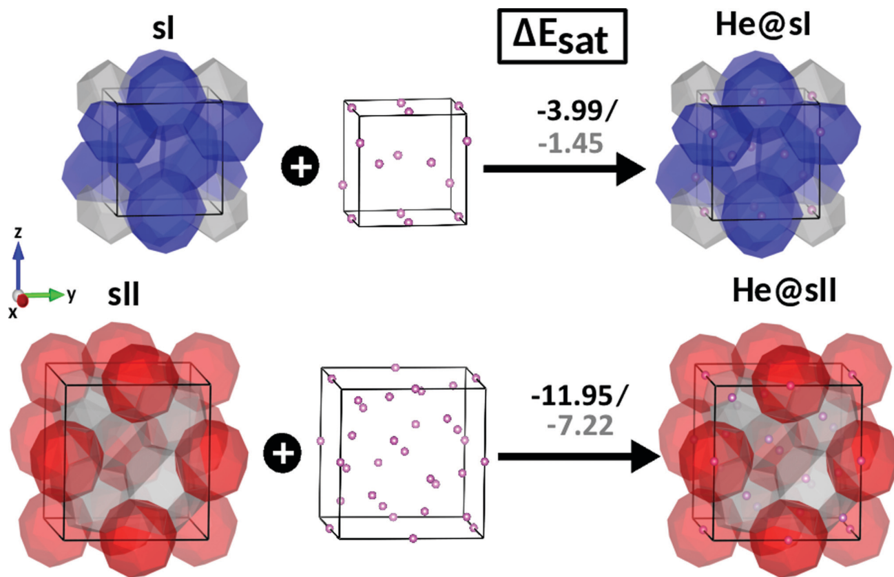
Fig. 5 Saturation energies, \Delta E_{\text{sat}} , in \text{kcal mol}^{-1} , for fully single cage occupation He@sl and He@sII clathrate hydrates, as computed from the present PW86PBE-XDM/D4 calculations.
