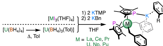
Scheme 2 Synthesis of complexes 6M ( \text{R} = \text{Me} ; \text{M} = \text{La}, \text{Ce}, \text{Pr}, \text{U}, \text{Np}, \text{Pu} ) and 7M ( \text{R} = \text{H} , \text{M} = \text{U}, \text{Np}, \text{Pu} ).
