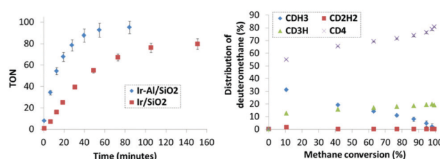
Fig. 4 Monitoring catalytic H/D exchange of methane. Left: Turnover number as a function of reaction time for catalysts Ir-Al/SiO 2 and Ir/SiO 2 at 250 °C and 0.67 mol% Ir surface sites. Right: Distribution of deuteromethanes as a function of CH 4 conversion for Ir-Al/SiO 2 .
