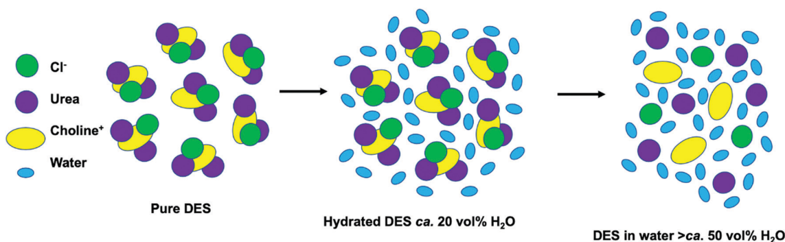
Fig. 16 Cartoon diagram showing structural changes in a DES starting with the pure choline Cl:urea DES (left). As the water content increases the hydrated DES regime is reached (middle, ca. 20 vol%), then the high concentration regime where everything is fully hydrated (ca. 50 vol%). Reprinted with permission from Elsevier. 207
