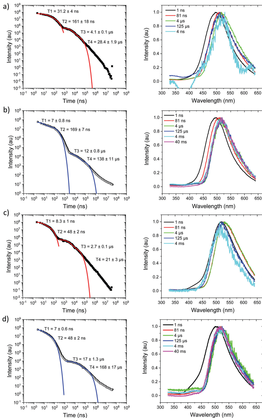
Fig. 6 Time-resolved spectrally integrated intensity decay (left) and representative time resolved spectra (right) of Ph 3 TRZCzTPA (a) 300 K and (b) 80 K; Ph 2 TRZCzTPA (c) 300 K and (d) 80 K in DPEO host. Spectral times given in ns, and decay fitting data included in the decay plots.
